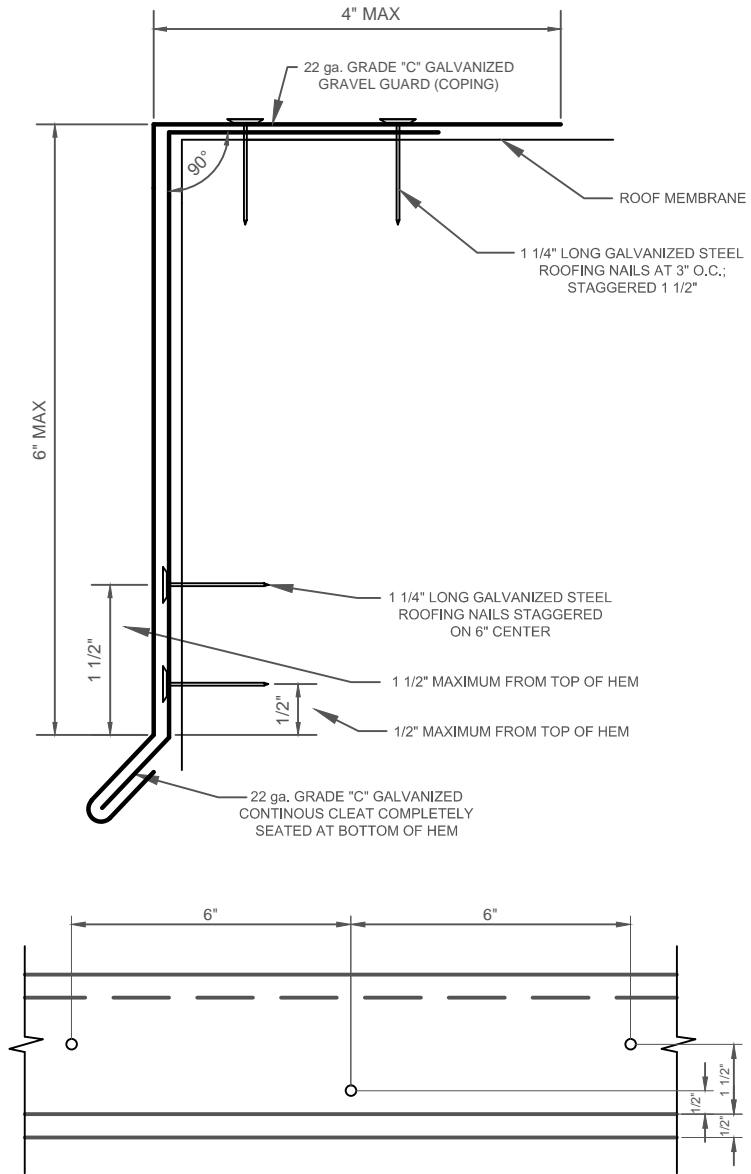
CONTINUOUS CLEAT
